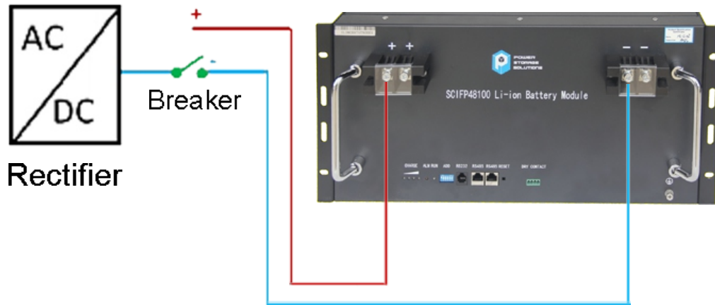
Figure 5-2: Single Battery Connection
