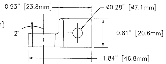
POST TERMINAL DETAIL (0.25" [6.4mm] THICK)
