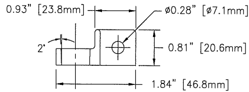
POST TERMINAL DETAIL (0.25" [6.4mm] THICK)
