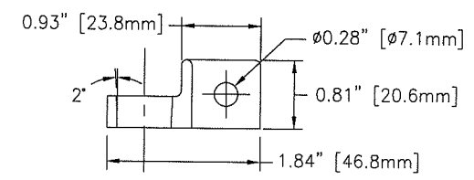
POST TERMINAL DETAIL (0.25" [6.4mm] THICK)
