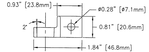
POST TERMINAL DETAIL (0.25" [6.4mm] THICK)
