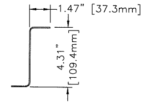
INTER-UNIT CONNECTOR PK02335
