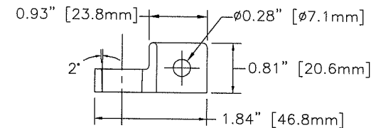
POST TERMINAL DETAIL (0.25\"/>
