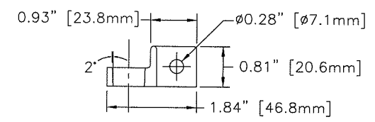
POST TERMINAL DETAIL (0.25" [6.4mm] THICK)
