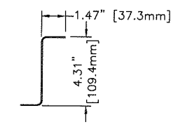
INTER-UNIT CONNECTOR PK02335
