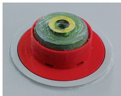
Fig. 5-15: Exemplary touch protection ring for GroE (similar to grid | power v_M )
