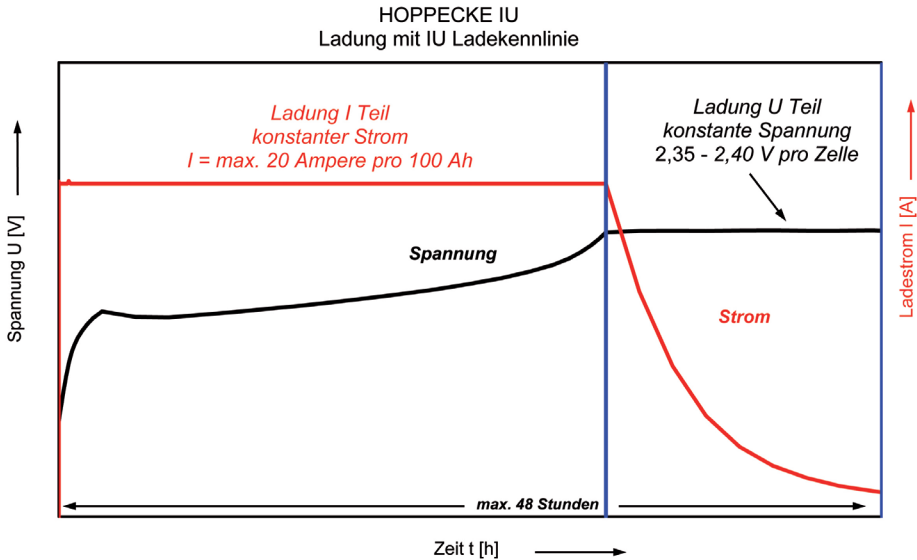
Fig. 9-1: IU characteristic
