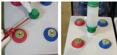
Fig. 5-21: Labyrinth plug (left) and grid | AquaGen recombination system (right)
