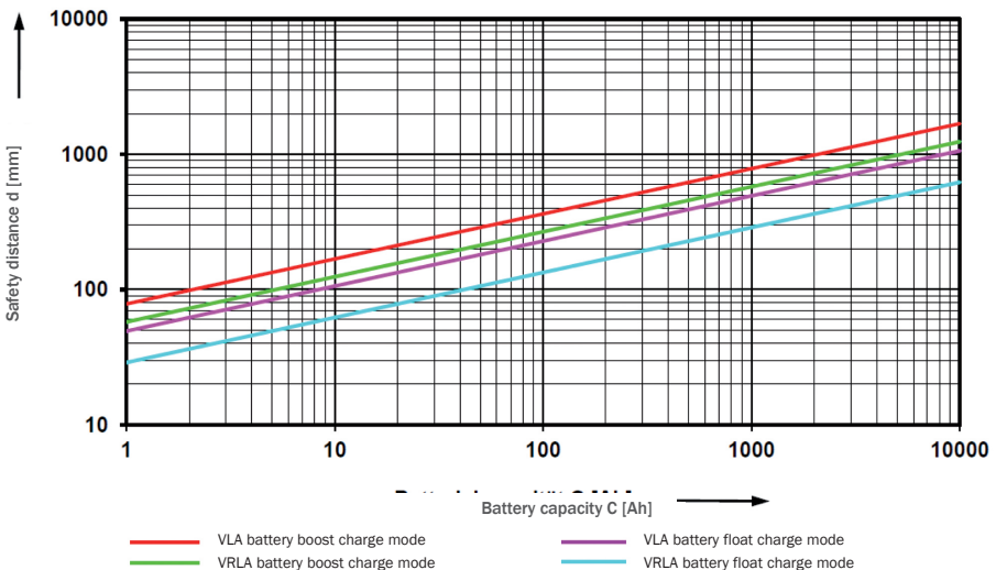
Fig. 5-1: Safety distance based on battery capacity
