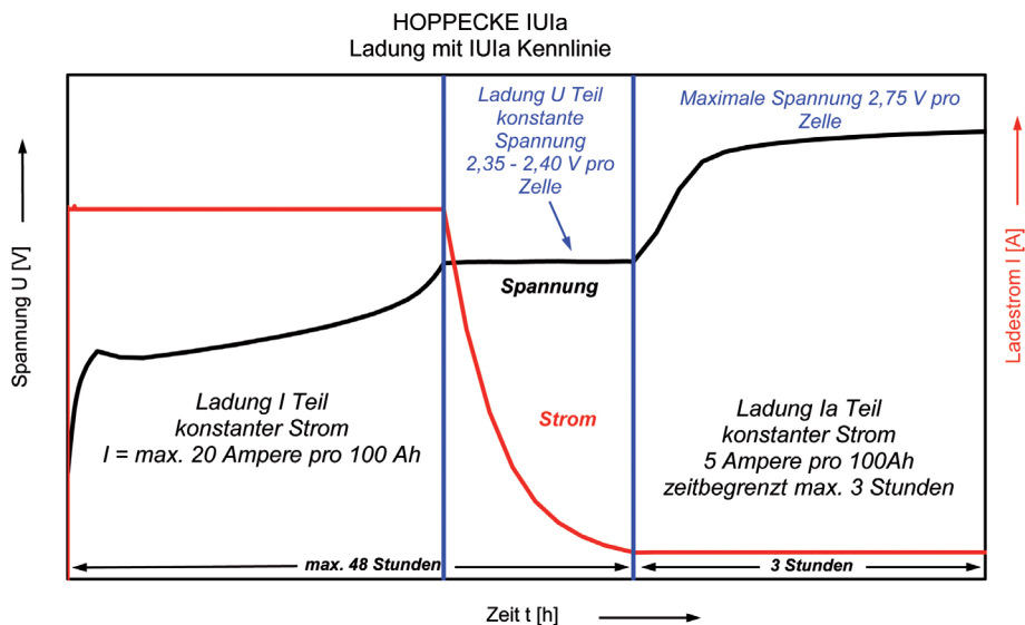
Fig. 9-2: IU la characteristic
