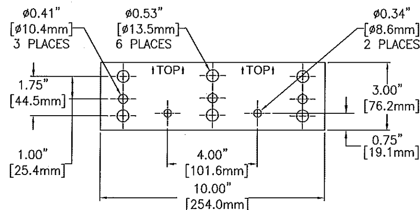
TERMINAL PLATE DETAIL PART NO. PT00959T
