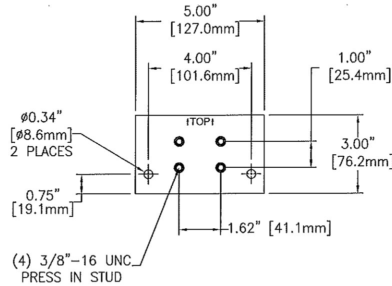
TERMINAL PLATE DETAIL PART NO. PT00963T
