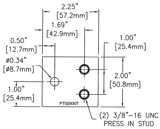
TERMINAL PLATE DETAIL PART NO. PT00930T
